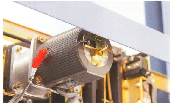
Independence induction motor with tension sensor for secondary tensioning.
